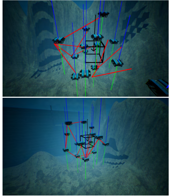
Fig. 4: 3D HoloOcean scene with multiple BlueROV2 vehicles during deployment under flow-driven dispersion. Red segments indicate pruned communication links within range R_{\max} . Top: View 1. Bottom: View 2.
